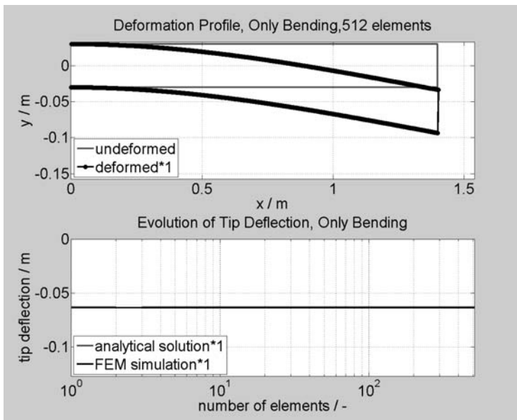
Figure 4: Timoshenko
