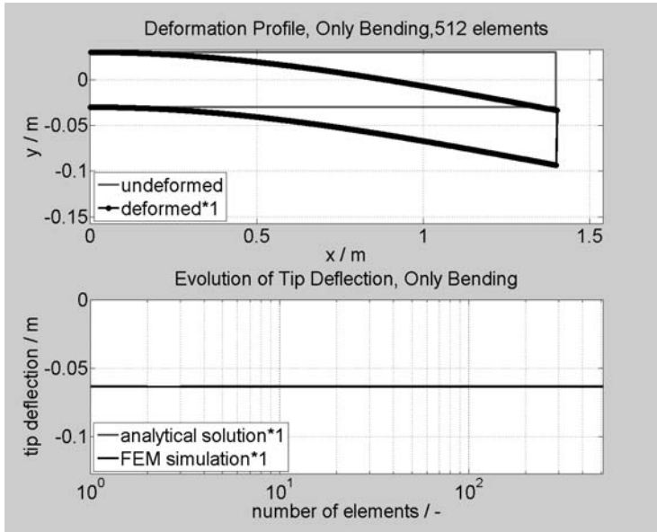
Figure 3: Only Bending
