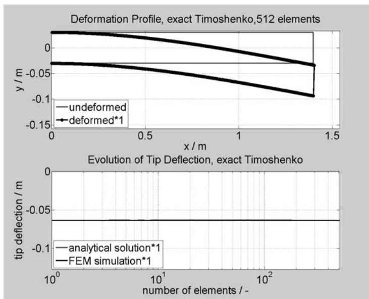
Figure 2: Exact Timoshenko
